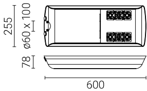
CUDDLE LED 48W, 60W, 72W
