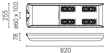
CUDDLE LED 96W, 120W, 144W
